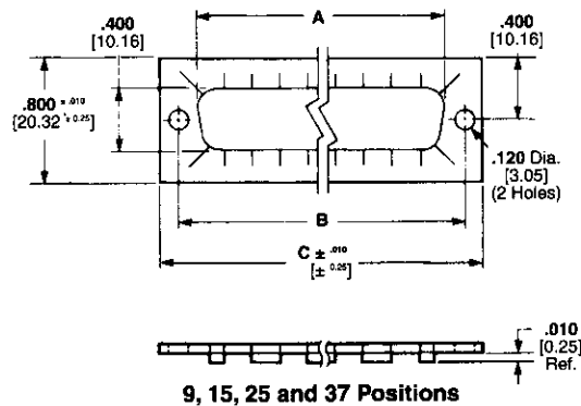
9, 15, 25 and 37 Positions
